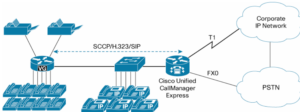
Figure 6. Cisco VG Integration with Cisco Unified Communications Manager Express
